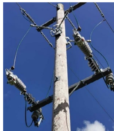
Single Phase Recloser
